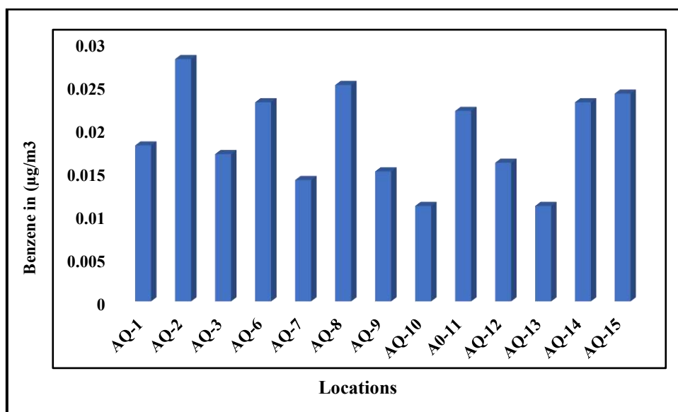
Fig – 2.7. Concentration of benzene air sample
