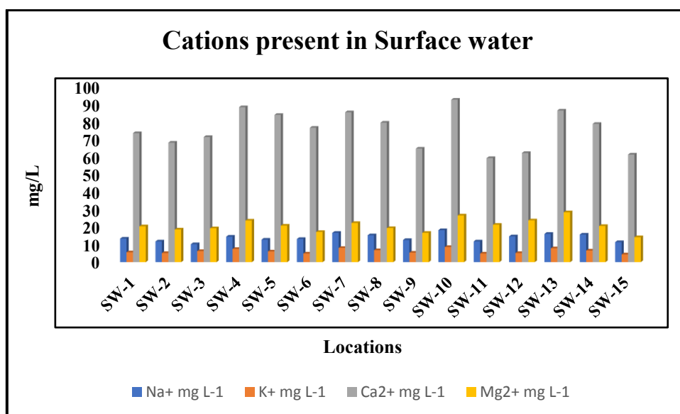
Fig. 2.14. Variation of cations in surface water sample
