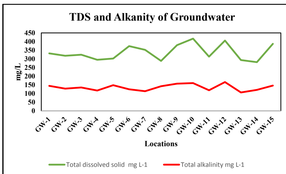
Fig. 2.19. Variation of TDS and alkanity in groundwater sample
